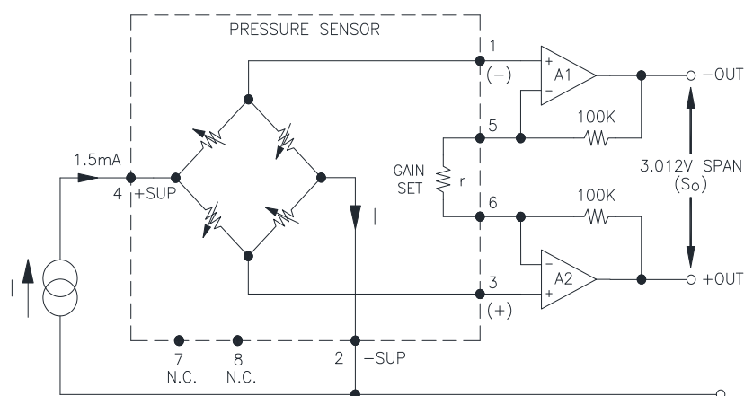
APPLICATION SCHFMATIC
